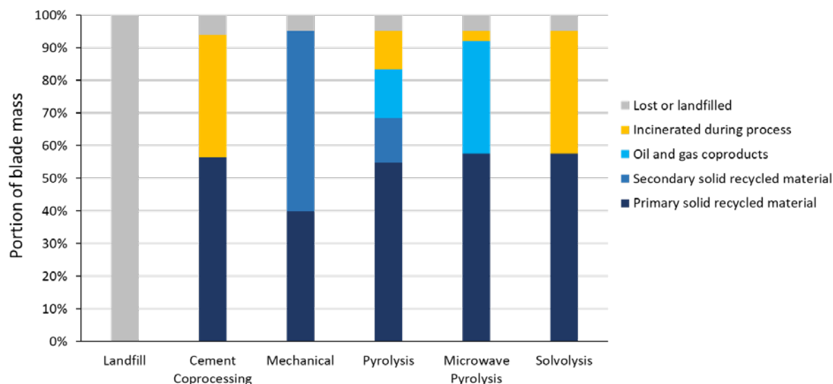
Figure 19. Wind turbine blade mass yields through different approaches. Figure by Evan Sproul, SNL.
